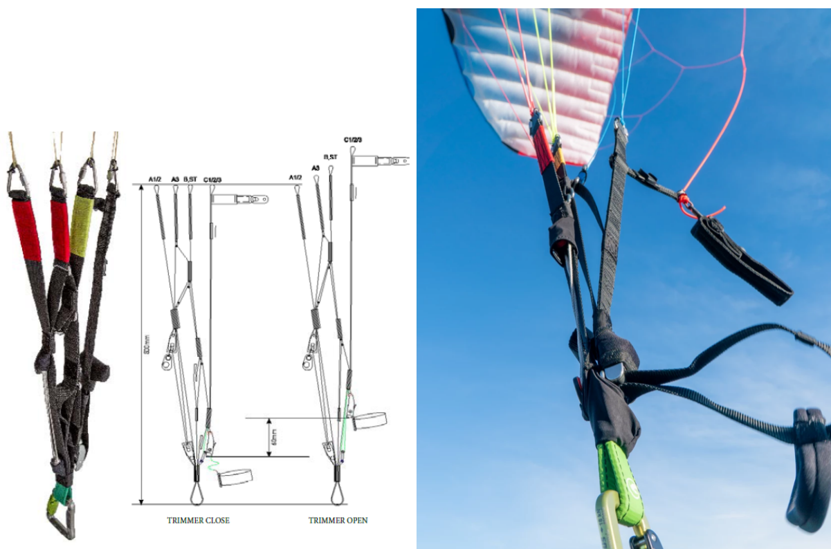
Illustration 10_ riserbelt
